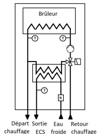
Figure 3 Chaudière murale à micro-accumulation double-service
