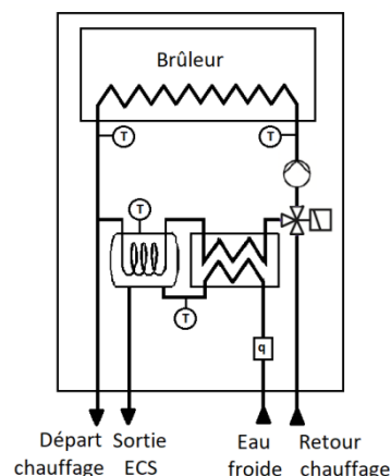
Figure 4 Chaudière murale à accumulation double-service
