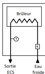
Figure 1 Chauffe-eau gaz instantané
