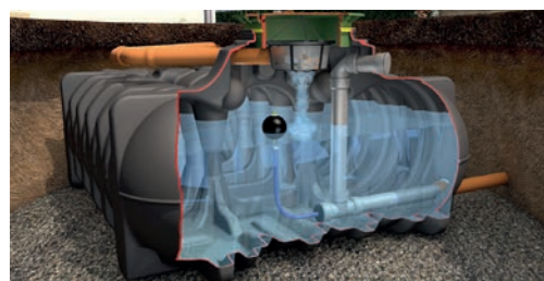
Cuves plates
